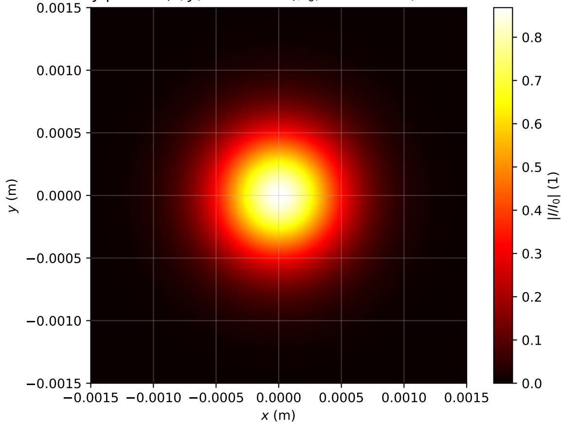
Intensity profile I(x, y, z = 1.513m)/I_0 , Pin=0.4Pcr, artificial time
